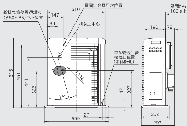
FFR-G5640SX
